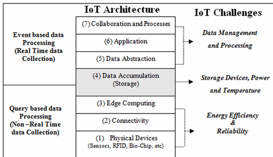
Figure 1. IoT World Form Reference Model
