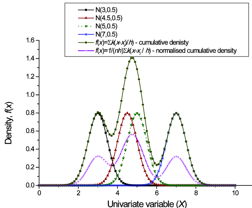
Figure 1. Kernel density estimation concept
