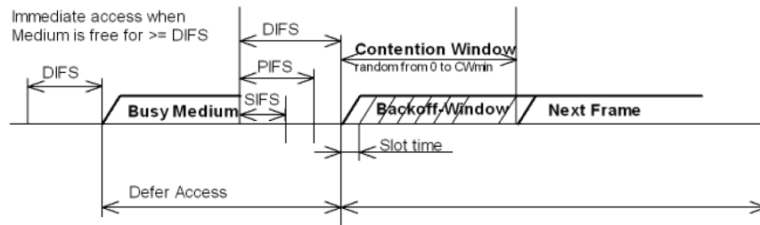
Figure 1. DCF access mechanism
