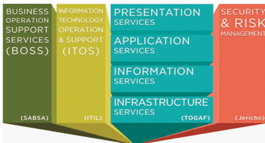
Figure 1. TCI reference architecture
